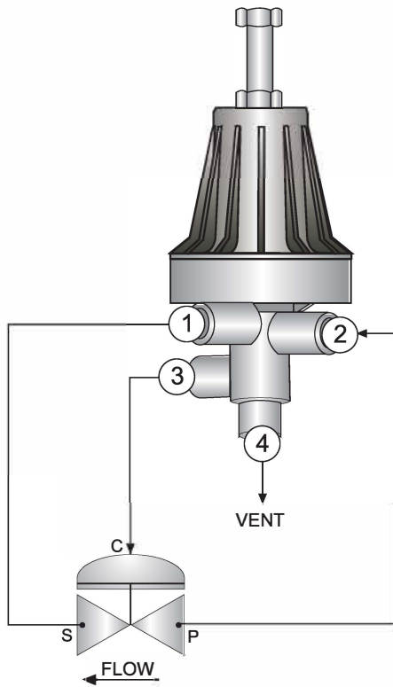
Pressure Reducing
