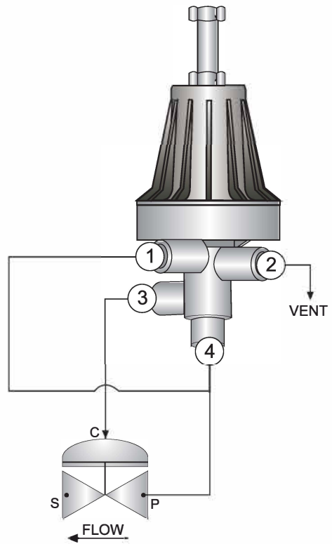
Pressure Sustaining
