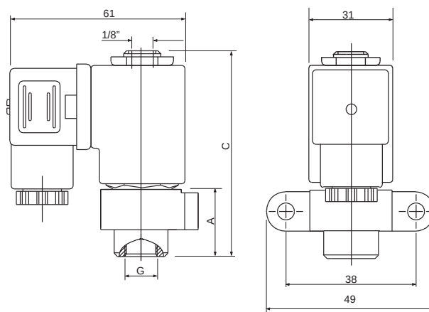
"INLINE" Mounting
