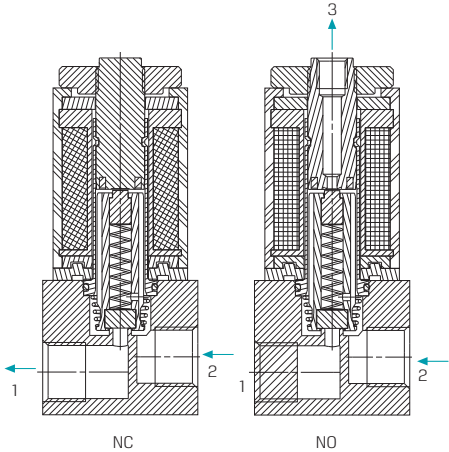
NC
